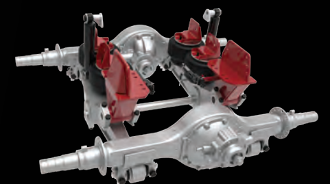
AIR LINK REDLINE WALKING BEAM
