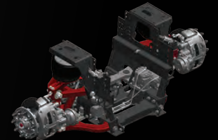
REYCO GRANNING IFS [20K AND 24K]
